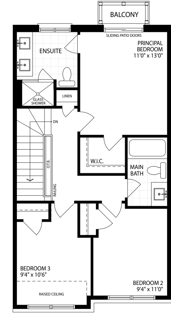
UPPER FLOOR ELEV. A
